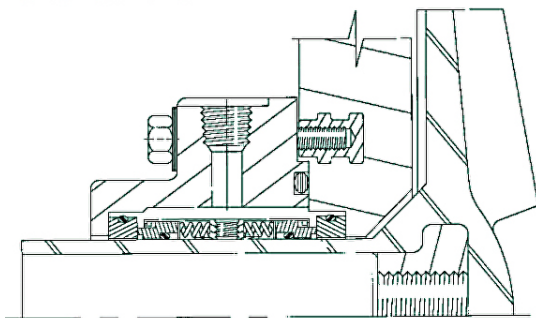
CRANE TYPE 8-1T
